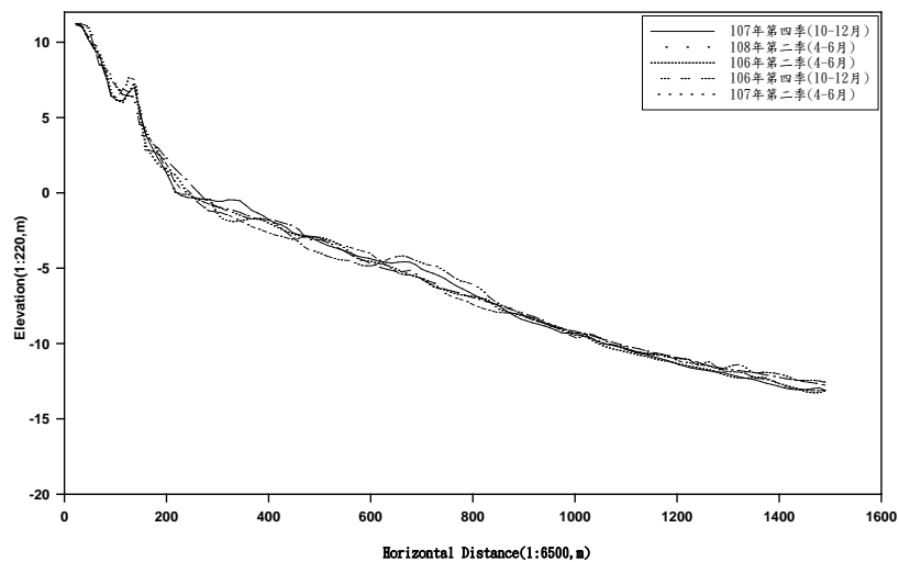
X-40 PROFILE
