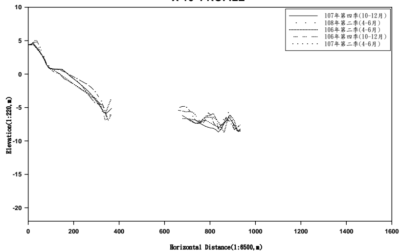
X-10 PROFILE
