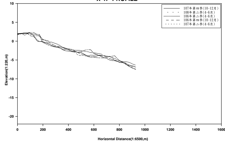
X-47 PROFILE
