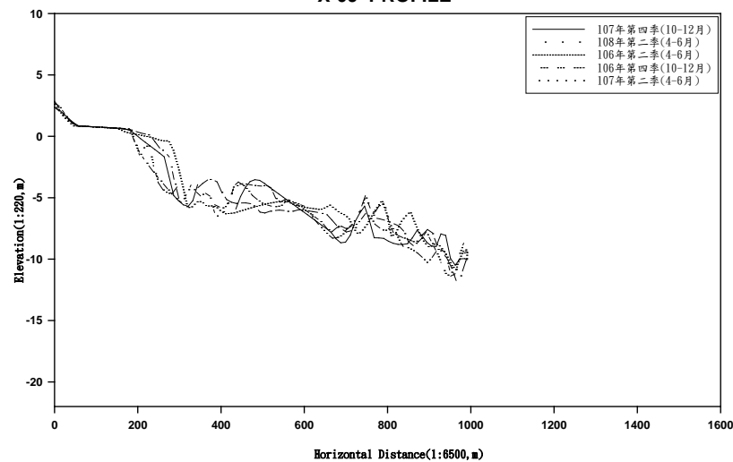
X-09 PROFILE
