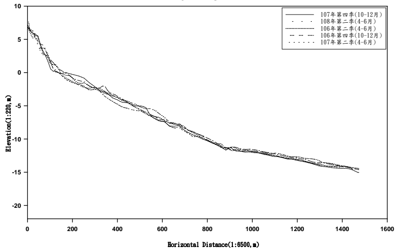
X-34 PROFILE
