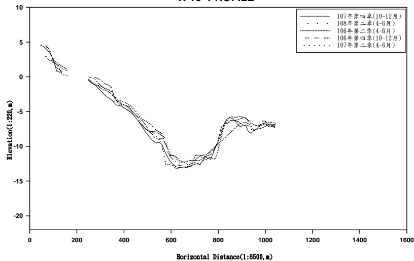
X-15 PROFILE
