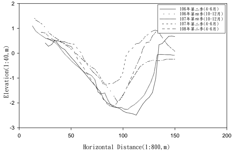
X-50 PROFILE
