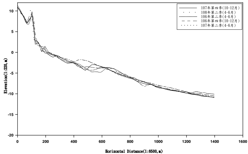
X-44 PROFILE
