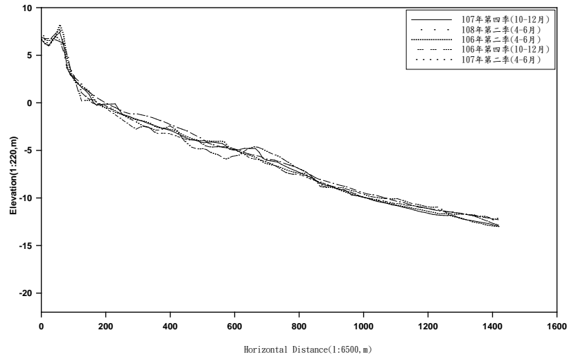
X-41 PROFILE
