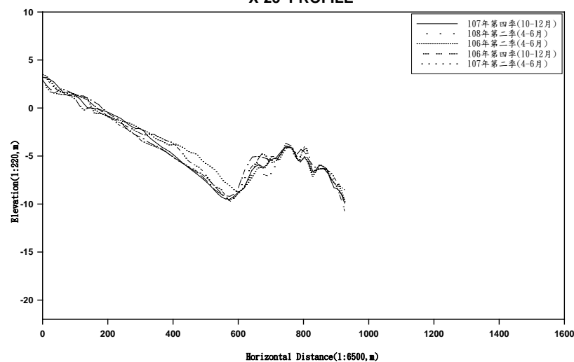
X-25 PROFILE
