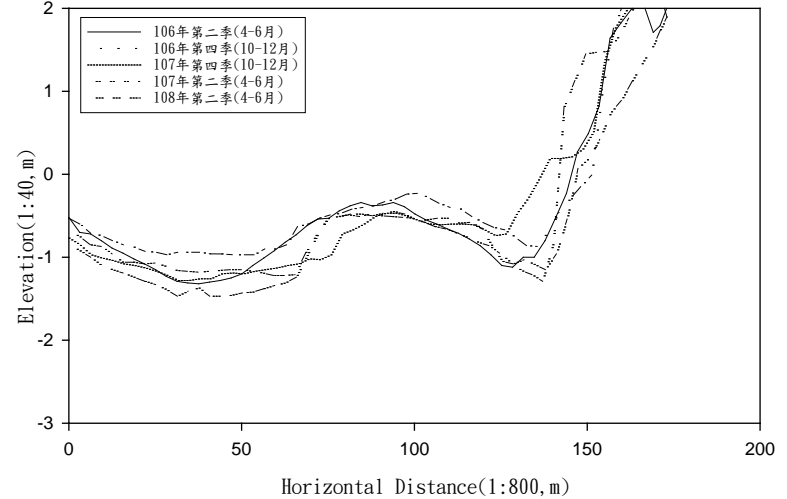
X-51 PROFILE
