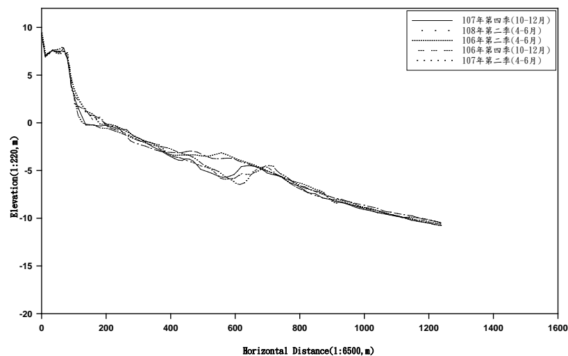
X-43 PROFILE
