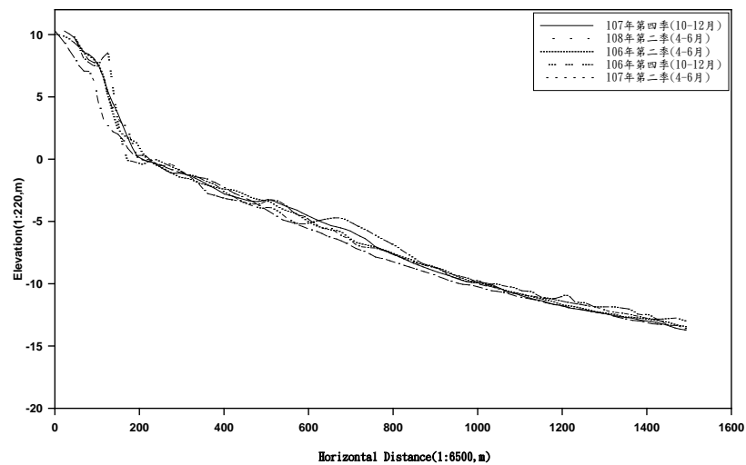
X-39 PROFILE
