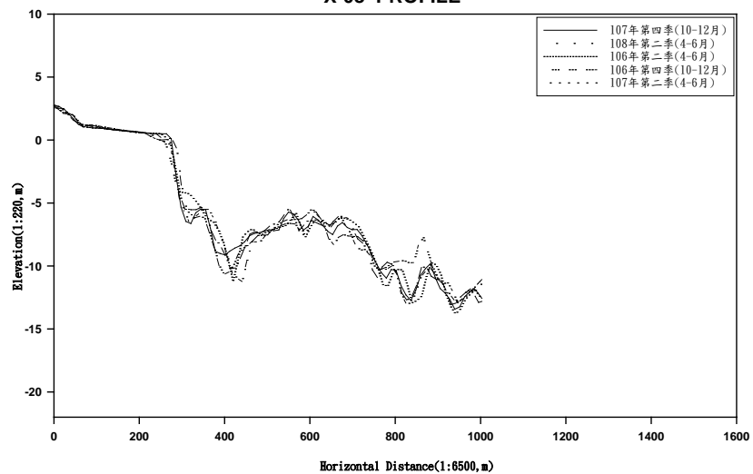
X-08 PROFILE
