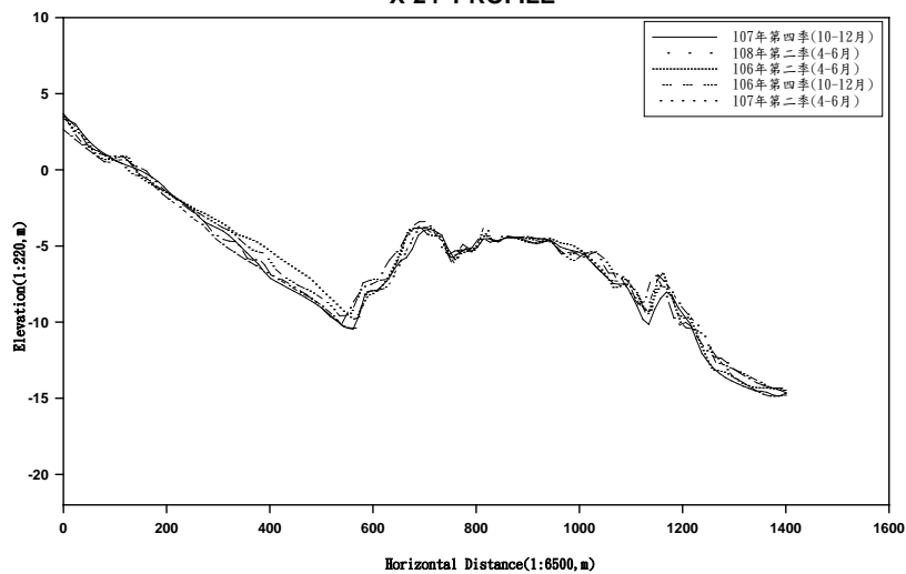
X-24 PROFILE
