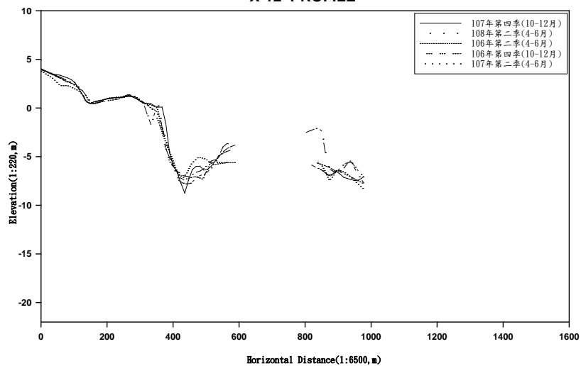
X-12 PROFILE
