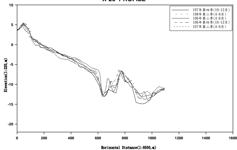
X-26 PROFILE
