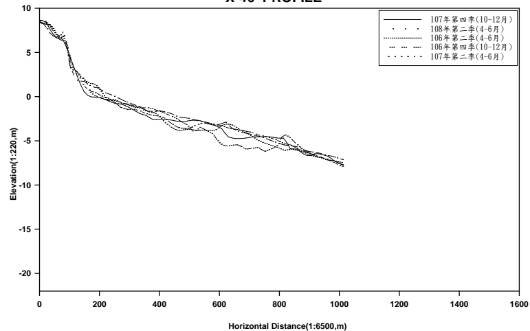
X-46 PROFILE
