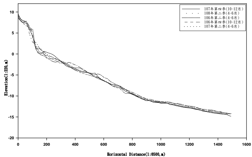
X-35 PROFILE
