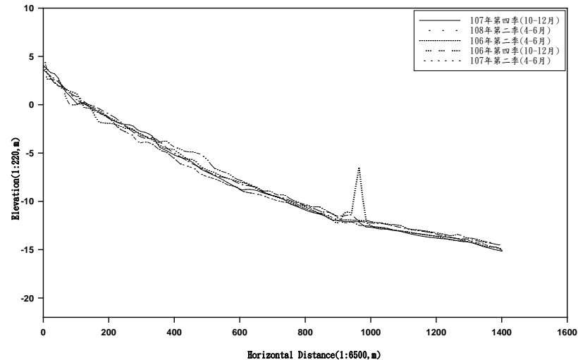
X-33 PROFILE
