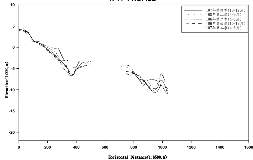
X-11 PROFILE
