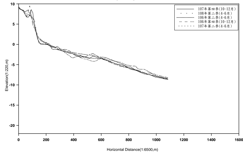
X-45 PROFILE
