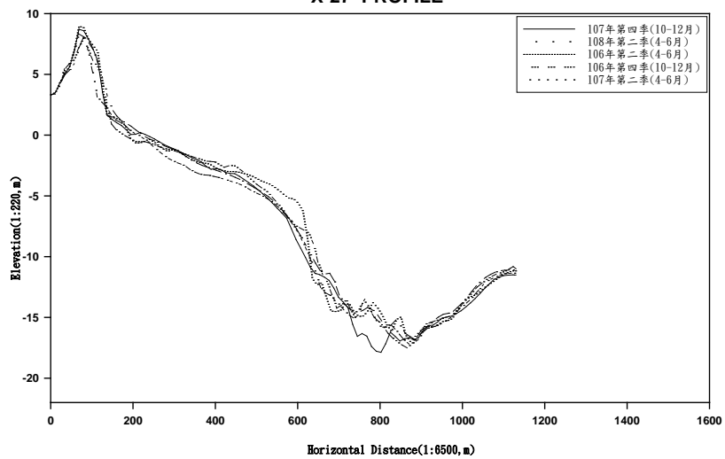
X-27 PROFILE
