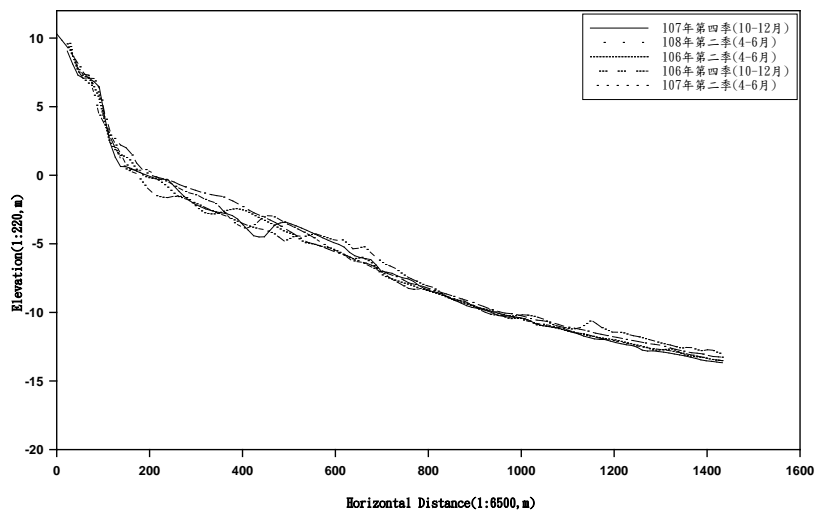
X-38 PROFILE
