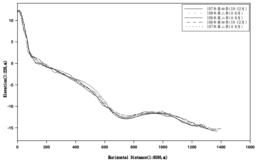
X-30 PROFILE
